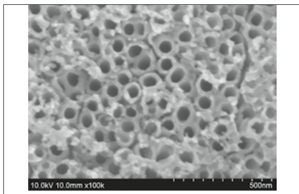
Figure 8. The surface of the photocatalyst \text{TiO}_2\text{NT}/\text{Au} at a magnification of 100.000 times.
