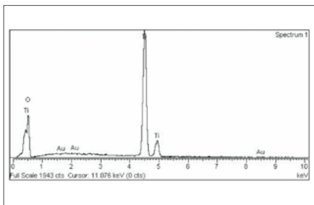
Figure 9. Elemental analysis (EDS) of photocatalyst \text{TiO}_2\text{NT}/\text{Au} .
